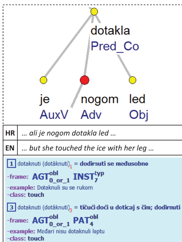
Figure 3. Treebank evidence and CROVALLEX frames for the verb dodirnuti (en. to touch )
